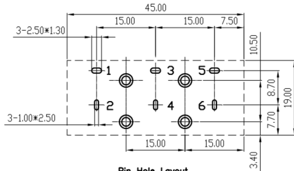
Pin Hole Layout (Jack Bottom View)
