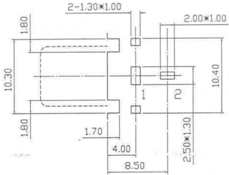
Pin Hole Playout Jack Bottom View
