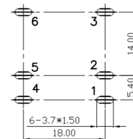
Pin Hole Layout (Jack Bottom View)
