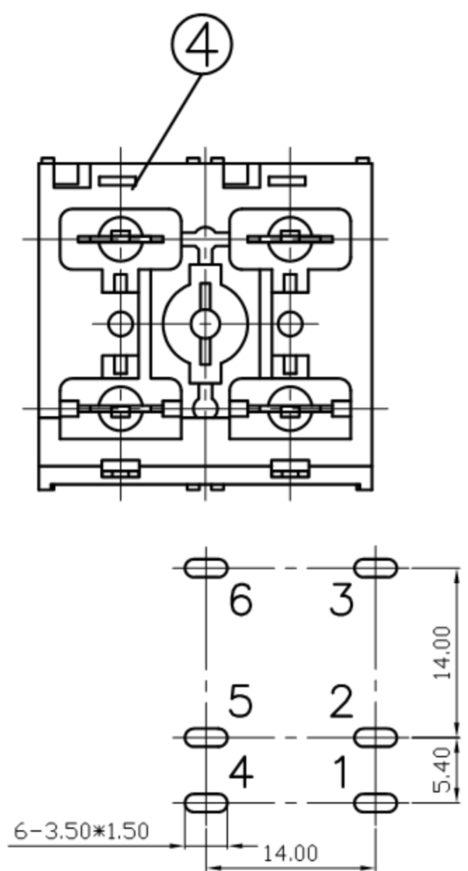
Pin Hole Layout (Jack Bottom View)
