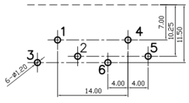
Pin Hole Layout (Jack Bottom View)
