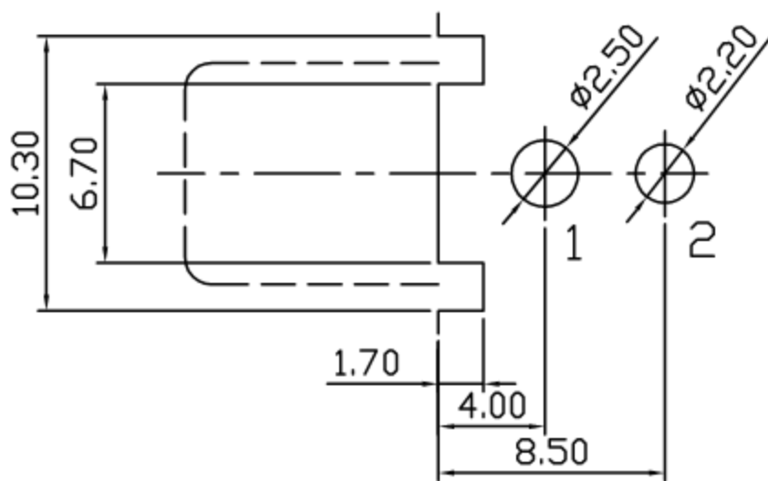
Pin Hole Layout (Jack Bottom View)
