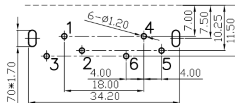
Pin Hole Layout (Jack Bottom View)
