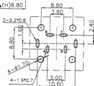
Pin Hole Layout (Jack Bottom View)
