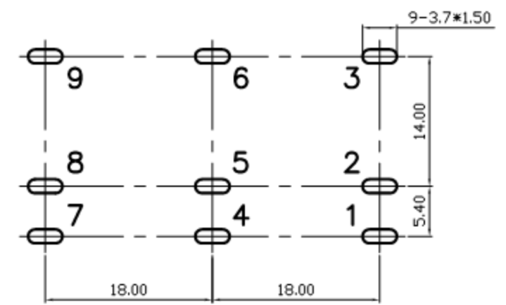
Pin Hole Layout (Jack Bottom View)
