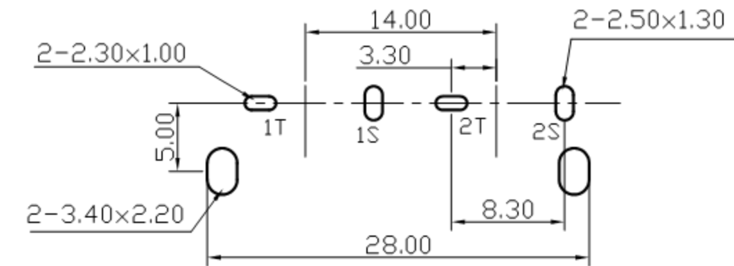
Pin Hole Layout (Jack Bottom View)
