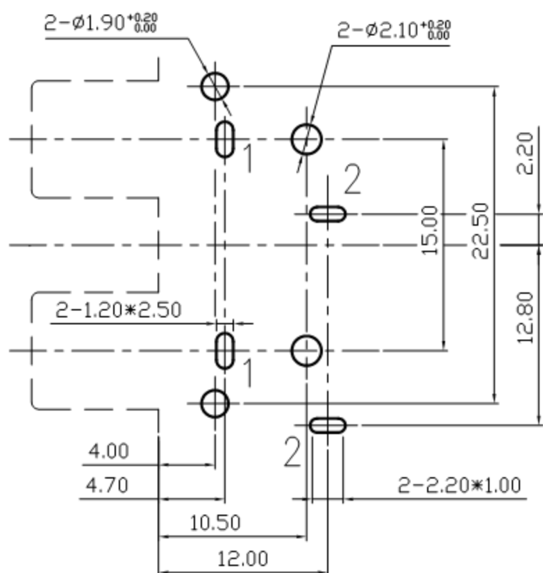
Pin Hole Layout (Jack Bottom View)
