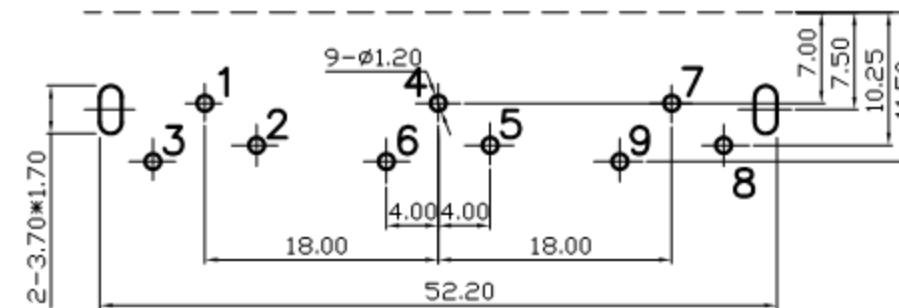
Pin Hole Layout (Jack Bottom View)
