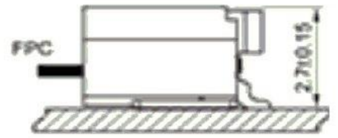
ASSEMBLY LAYOUT
