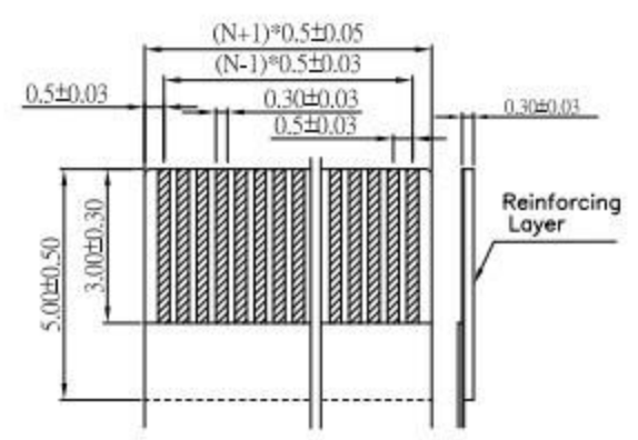
RECOMMENDED FFC/FPC DIM.
