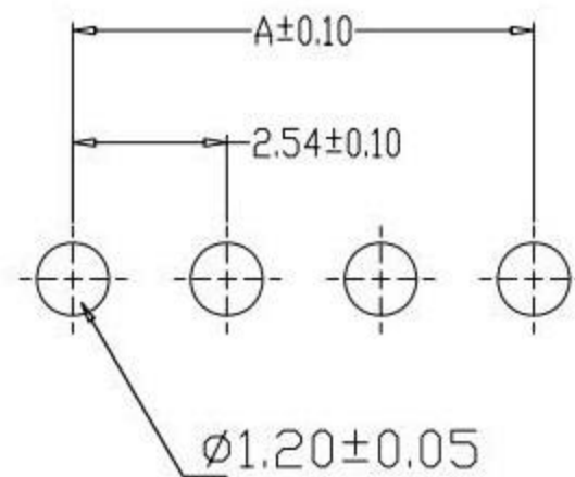
PCB LAYOUT
