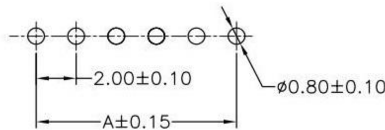
SUGGESTED PCB LAYOUT (COMPONENT SIDE)
