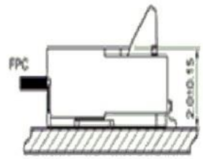
ASSEMBLY LAYOUT
