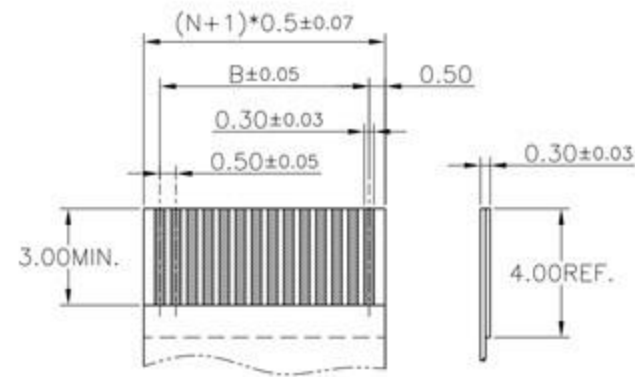
APPLICABLE FFC TOLERANCE:±0.05
