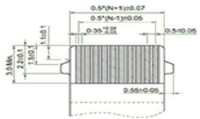
Applicable Flat Cable 1
