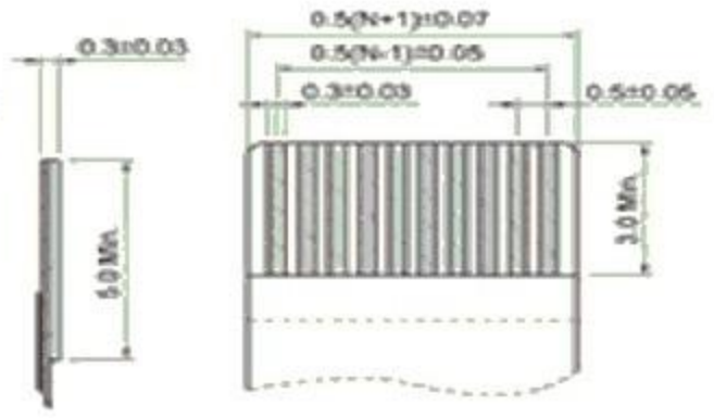
Applicable Flat Cable 2
