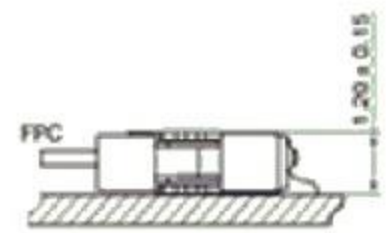
ASSEMBLY LAYOUT
