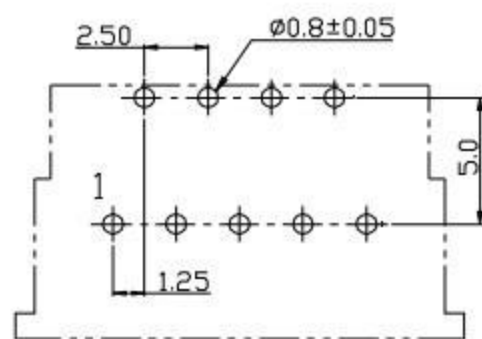
RECOMMEND PCB LAYOUT COMPONENT SIDE (FOR:GS15-XX1XA)
