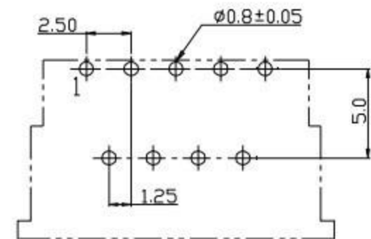
RECOMMEND PCB LAYOUT COMPONENT SIDE (FOR:GS15-XX1XAW)
