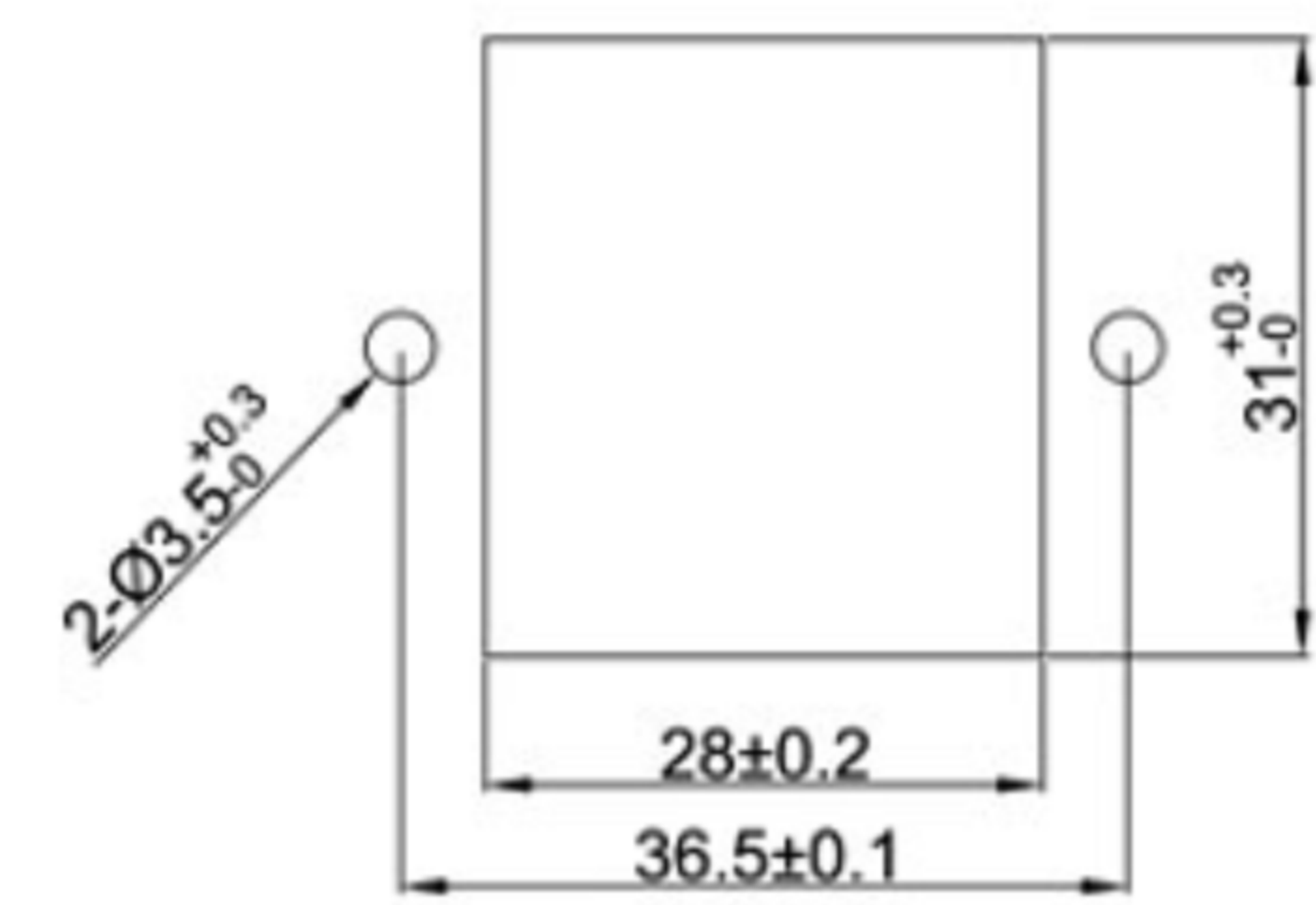
PANEL CUTOUT
