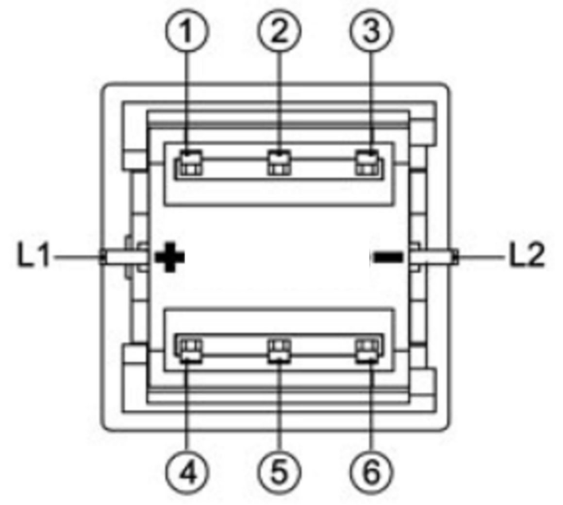
Bottom View
