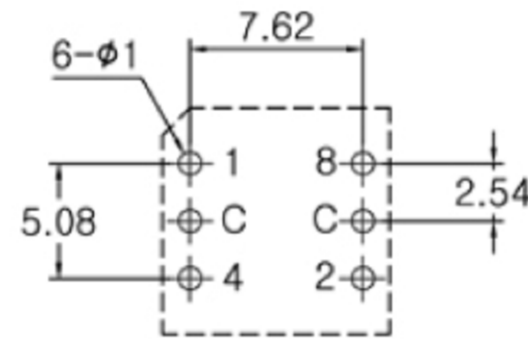
P.C.B DIMENSION (Top View)
