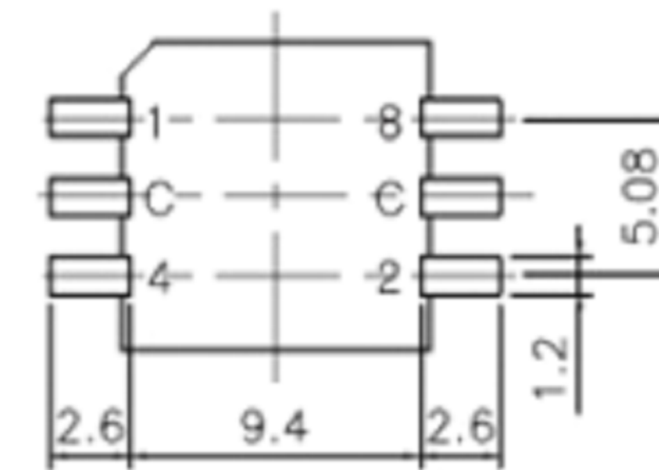
P.C.B DIMENSION (TOP VIEW)
