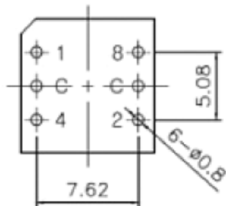
P.C.B DIMENSION (TOP VIEW)
