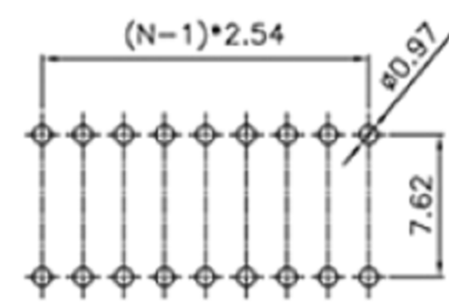
PCB LAYOUT
