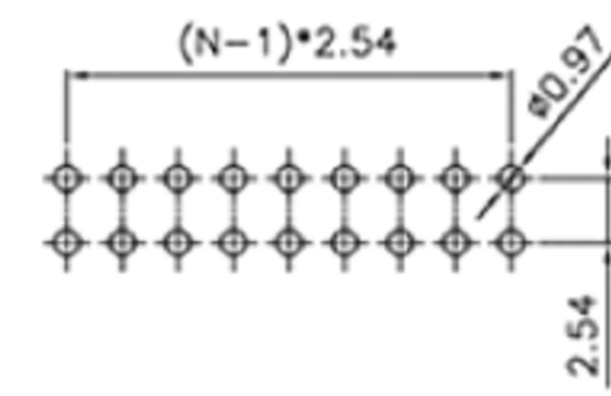
PCB LAYOUT
