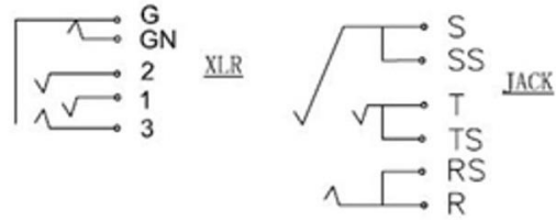
CONTACT SCHEMATIC CHART
