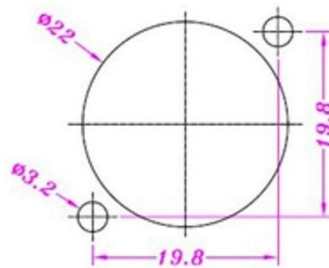
Panel cut out (rear side)
