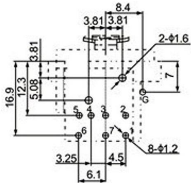
PC.B LAYOUT (VIEWED FROM COPPER SIDE)
