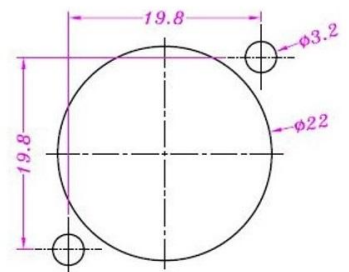
PANEL CUTOUT DETAIL
