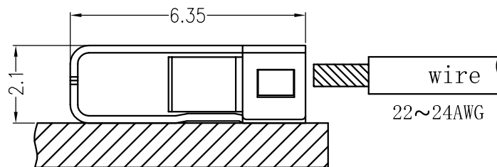
Assembly Layout
