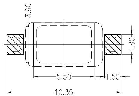
Board Layout General Tolerance: \pm 0.05
