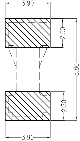
Board Layout
