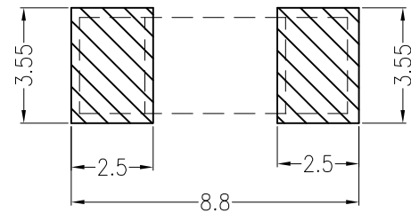
Board Layout
