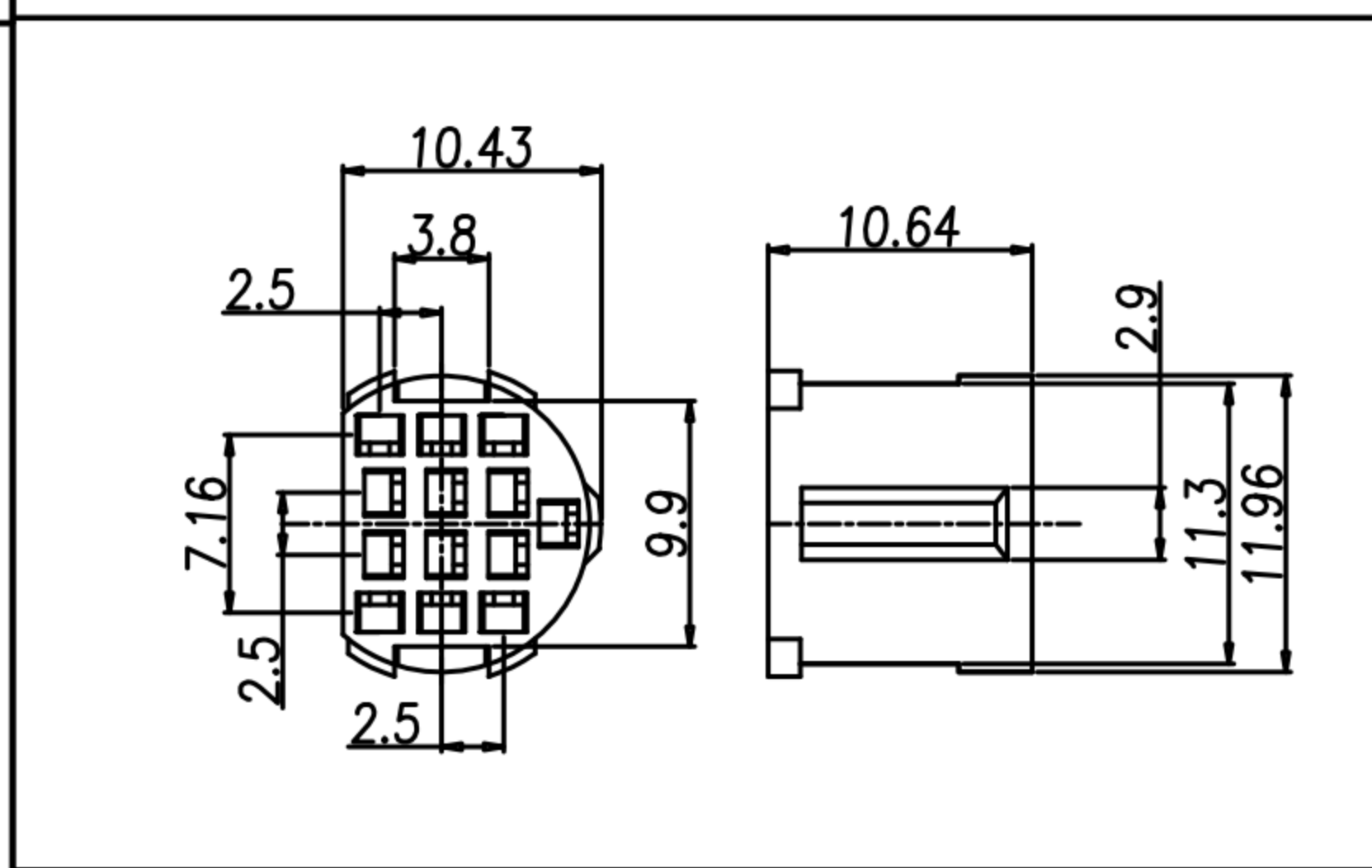
DN-DM0024(HOUSING)
