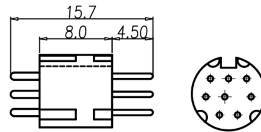
8PIN HOUSING+PIN
