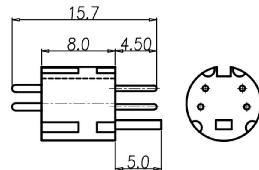
4PIN HOUSING+PIN
