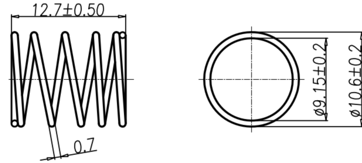
OS-DM0011 LOCK SPRING
