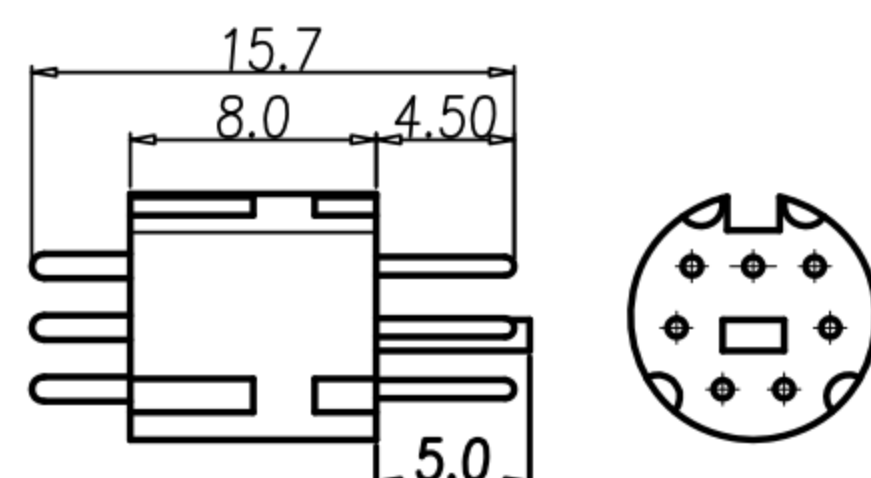
7PIN HOUSING+PIN
