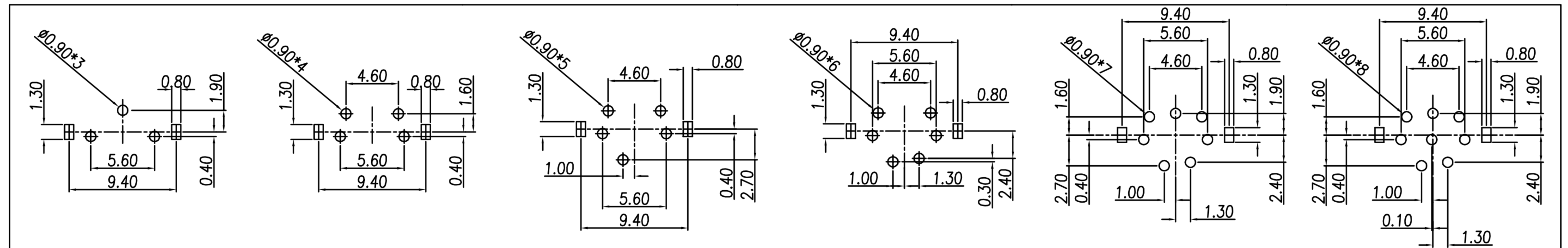
P.C.B LAYOUT (Bottom View)
