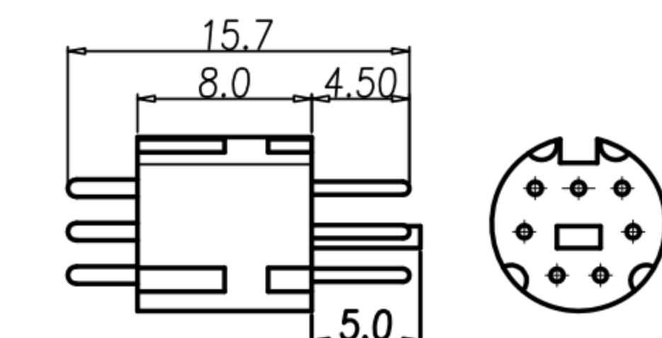
7PIN HOUSING+PIN
