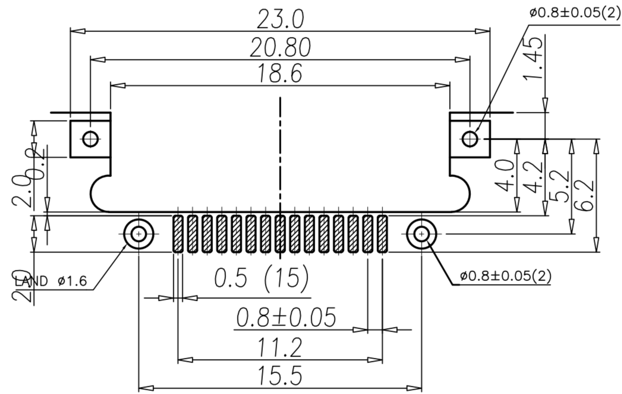
P.C.B LAYOUT TOP VIEW TOLERANCES:±0.1
