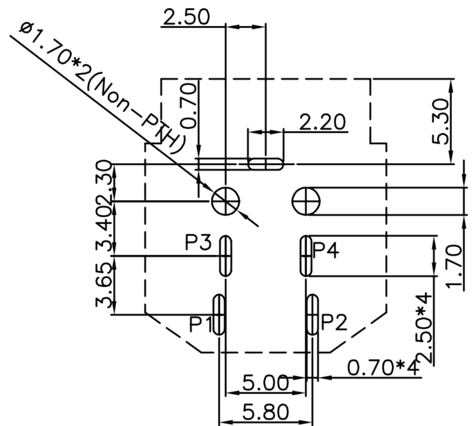
HOLE LAYOUT(BOTTOM VIEW)
