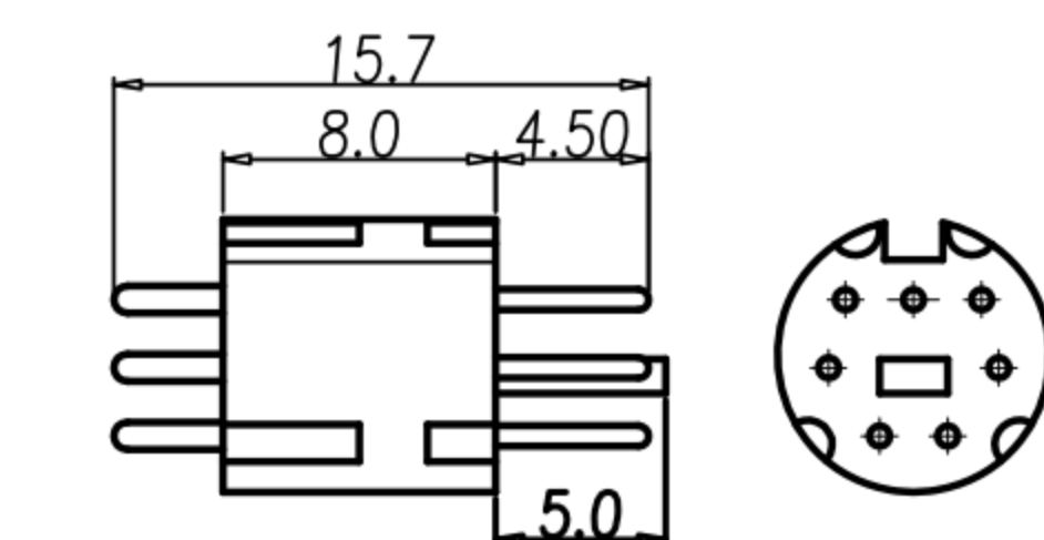
7PIN HOUSING+PIN
