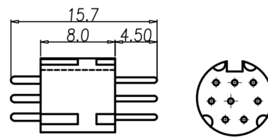
8PIN HOUSING+PIN
