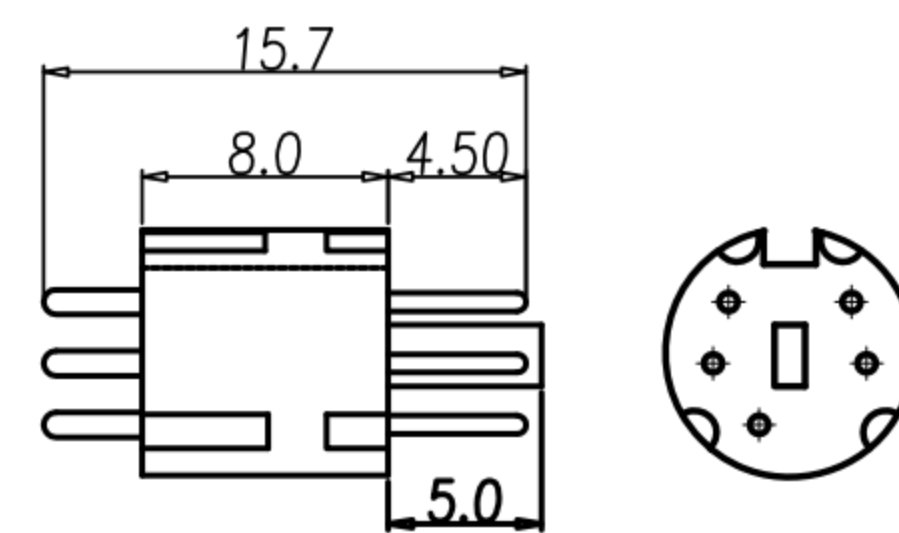
5PIN HOUSING+PIN
