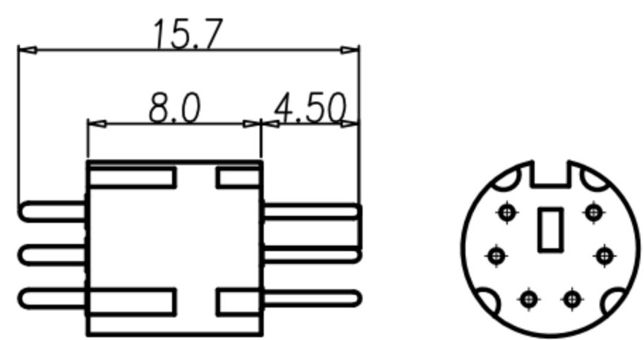
6PIN HOUSING+PIN
