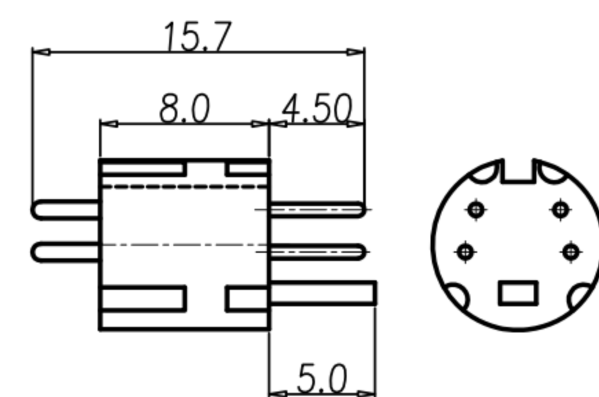
4PIN HOUSING+PIN
