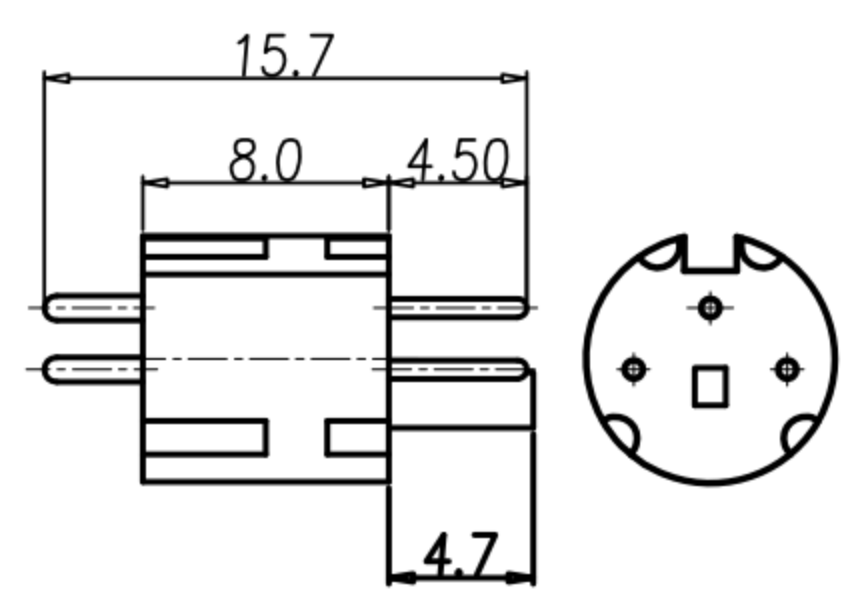
3PIN HOUSING+PIN
