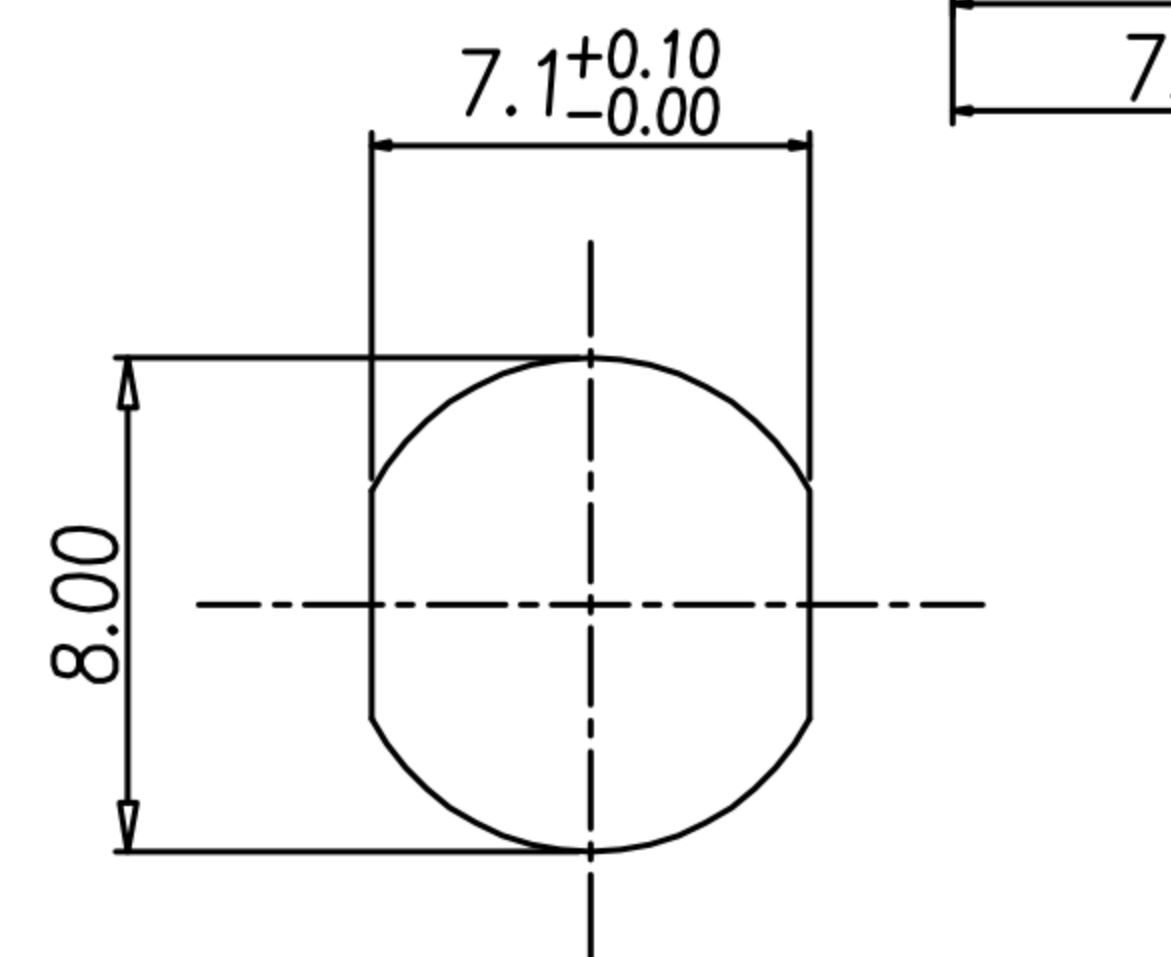
RECOMMENDPANEL CUT-OUT
