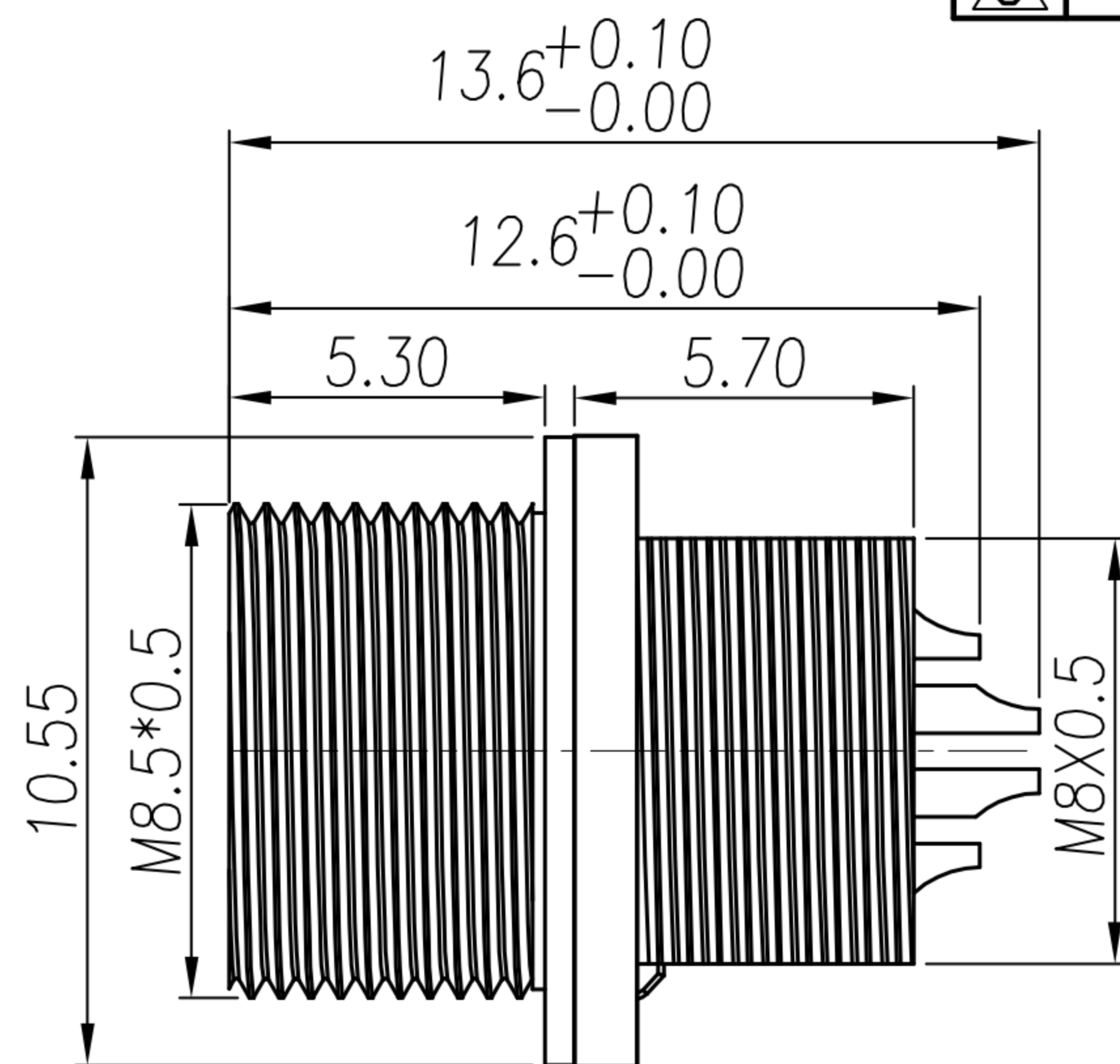
HOUSING+CONTACT+SHELL+O-RING
