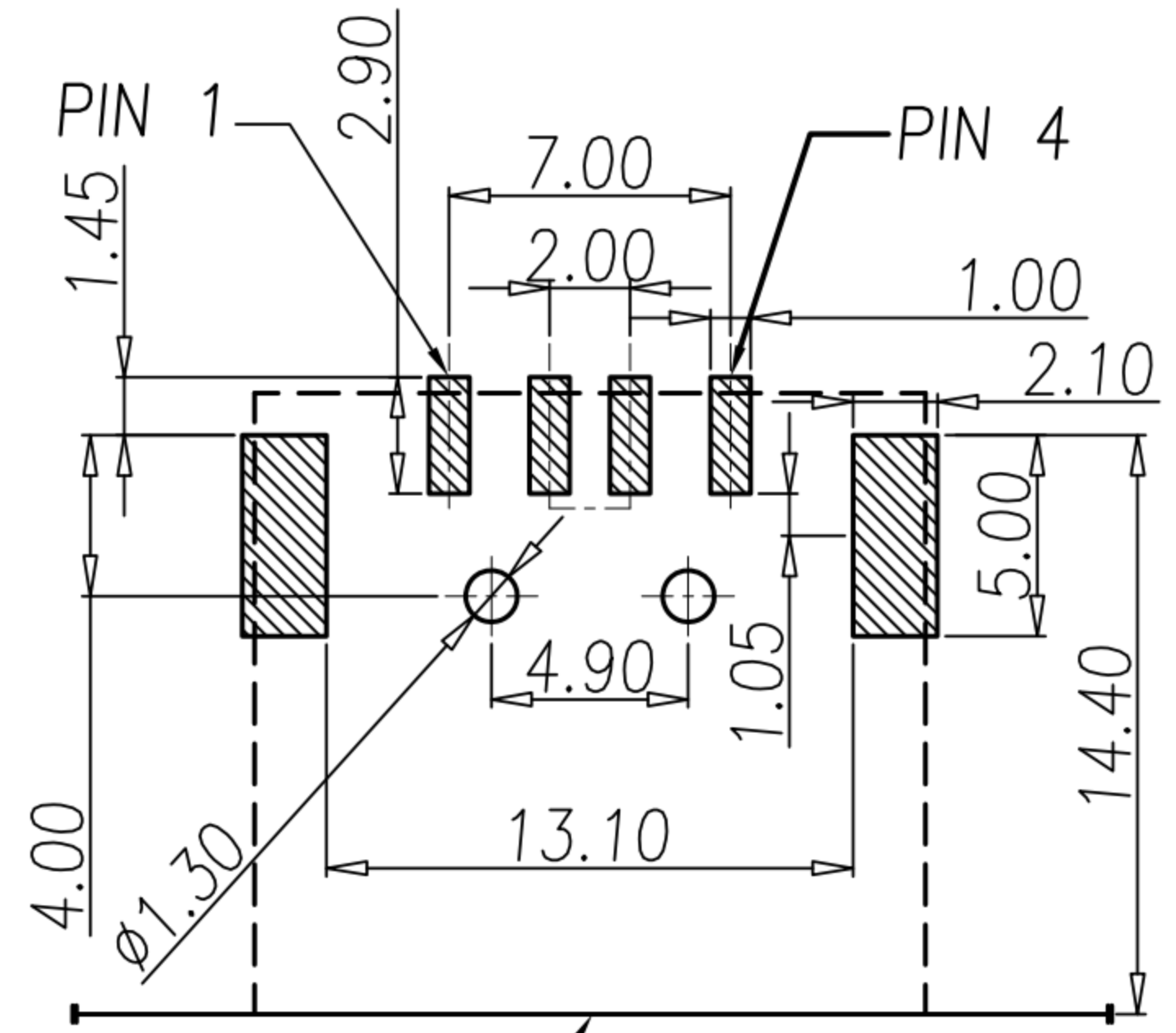
P.C.B. COMPONENT SIZE LAYOUT (TOP VIEW) TOLERANCE ±0.05 mm
