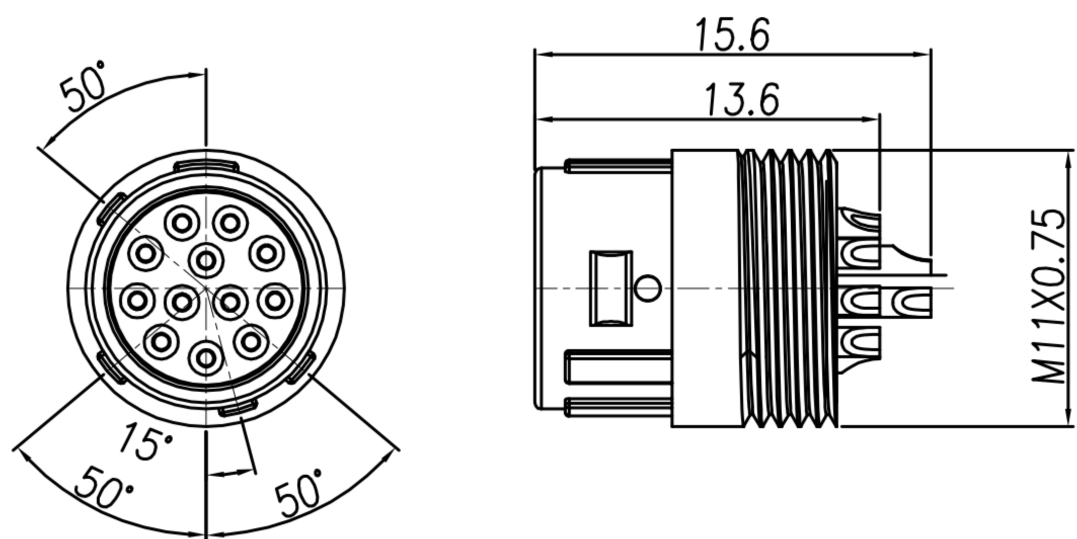
HOUSING + CONTACT + SHELL A
