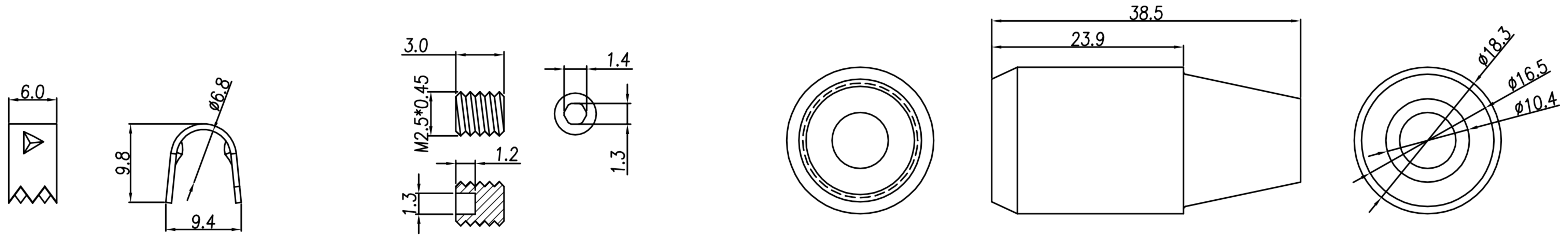
CLAMP
