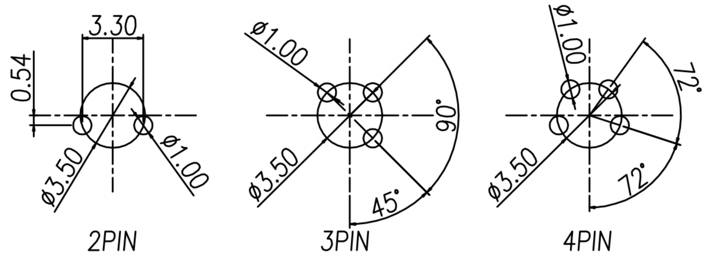
RECOMMEND PCB LAYOUT
