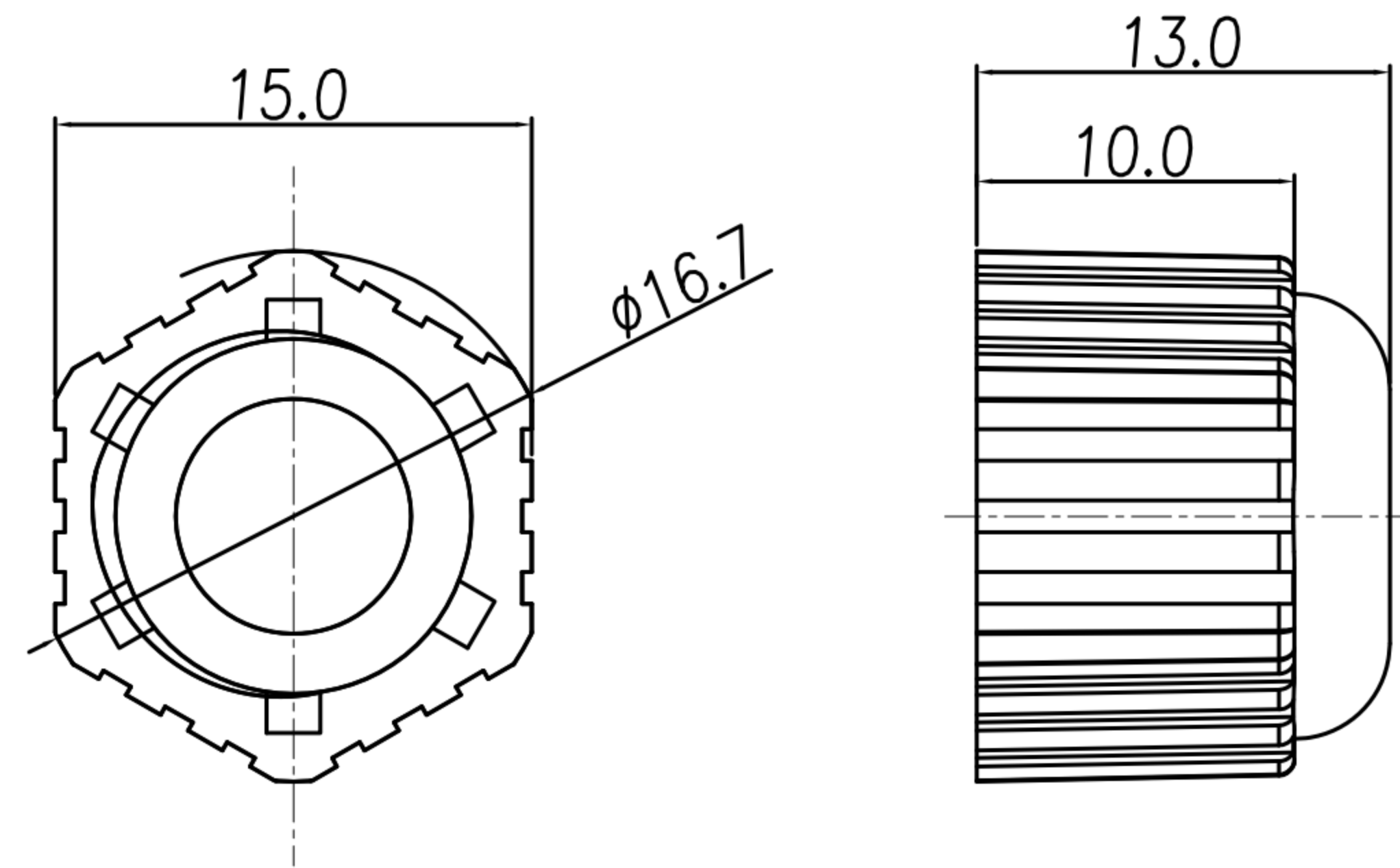
SEALING NUT
