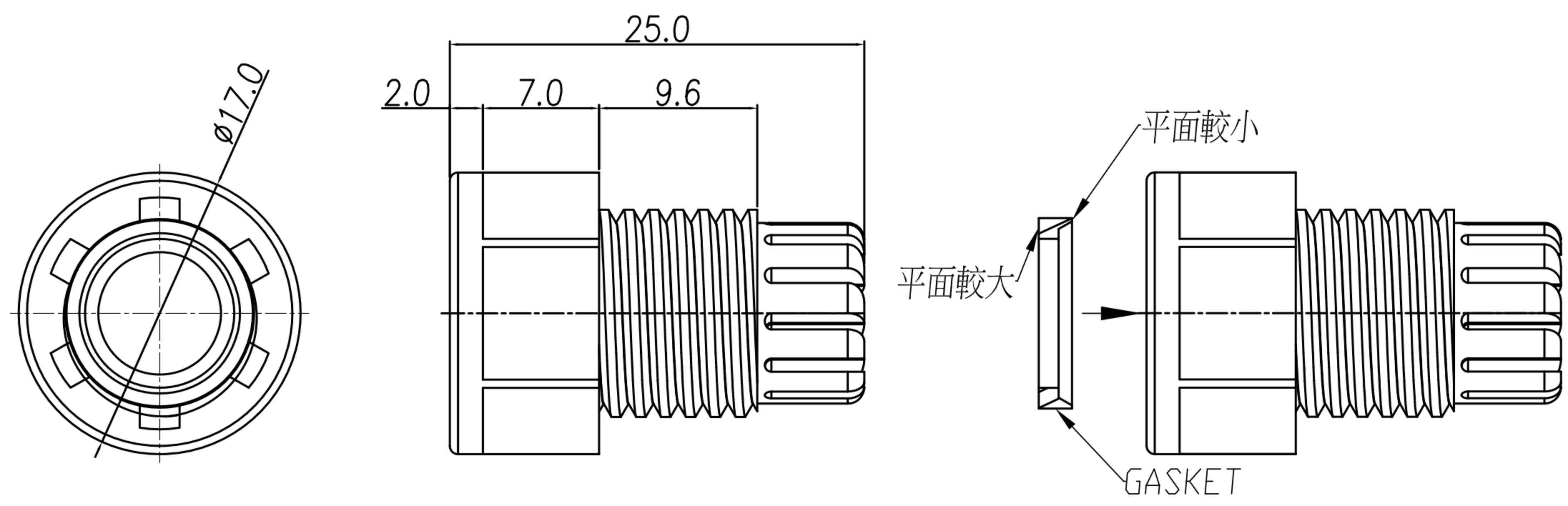
GASKET & CLAMP RING & SEAL
