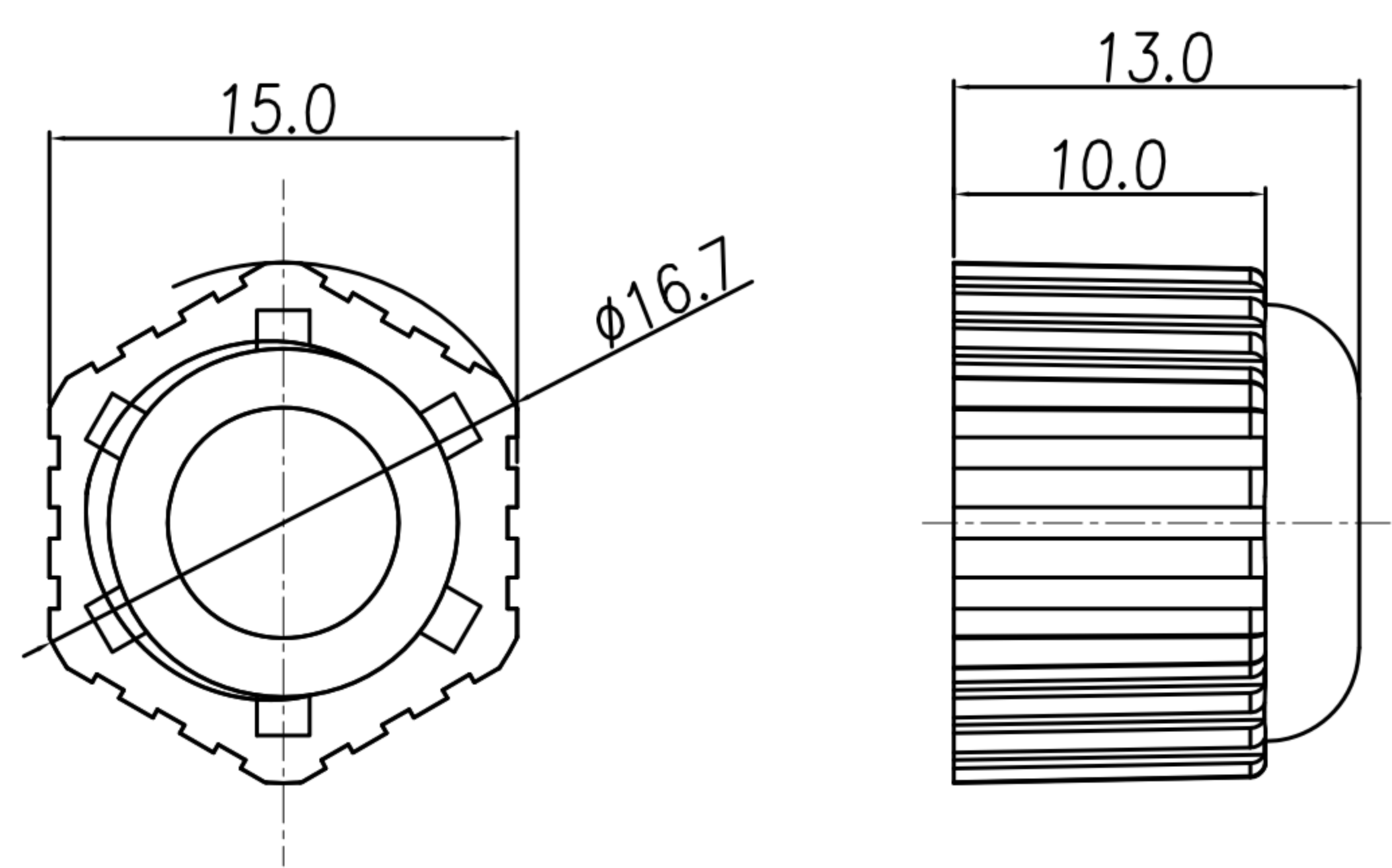
SEALING NUT
