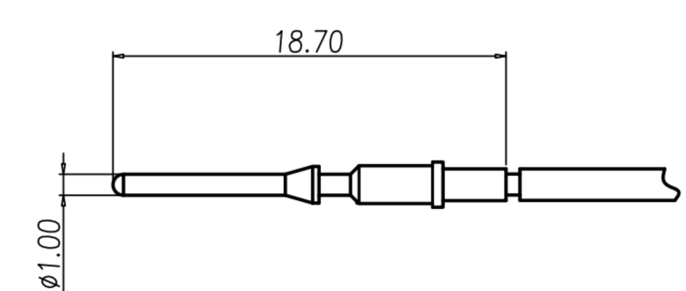
CONTACT ASS'Y FOR 24AWG~28AWG
